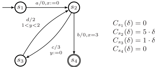
Fig. 1. The weighted timed automaton for Example 1
