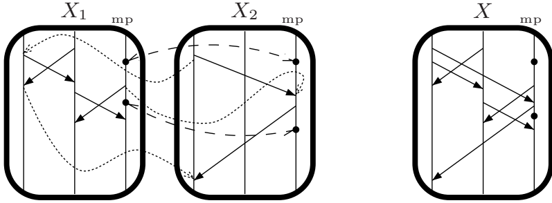
Fig. 4. X \in X^1 \parallel_{\text{mp}} X^2 and the corresponding relations \rightarrow^1 \cup \rightarrow^2, \leftrightarrow
