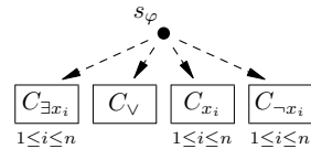
Fig. 10. Structure of modal specification (M_\varphi, s_\varphi) : \star -transitions lead from s_\varphi to components that detect possible flaws in potential valuation trees of \varphi
