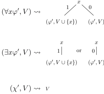
Fig. 6. Semantics of QCNF as a non-deterministic rewrite system
