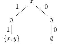
Fig. 7. Valuation tree witnessing the truth of \forall x \exists y (\neg x \vee y) \wedge (\neg y \vee x)
