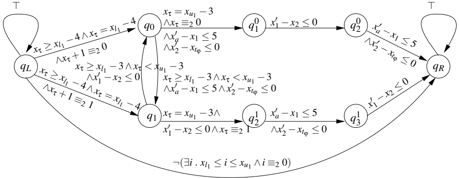
Fig. 3. The FBCA for the diagonal edges in the formula \phi : \forall i, j. l_1 \leq i \leq u_1 \wedge l_2 \leq j \leq u_2 \wedge i - j \leq 3 \wedge i \equiv 2 0 \wedge j \equiv 2 1 \rightarrow a[i] - b[j] \leq 5 from Fig. 2(a) obtained as D(a, t_\varphi, 3, 5, 2, 0 - 3, \{l_1 - 3\}, \{u_1 - 3\}, \text{left}) . To understand the formula \xi_0 on the transition from q_0 to q_1 , note that the constraint i \equiv_s k + t in the definition of the set K_0 instantiates to 0 \equiv_2 k - 3 , and hence K_0 = \{1, 3\} . A similar reasoning applies for the other transitions.
