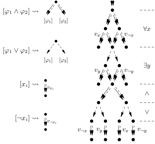
Fig. 11. Deterministic rules rewriting a QCNF formula \varphi into a specification (N_\varphi, t_\varphi)
